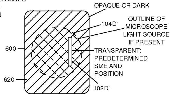
Fig. 10D-- OBLIQUE AND MODULATION CONTRAST ILLUMINATION
