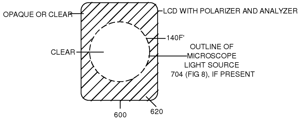
Fig. 10F--POLARIZED ILLUMINATION
