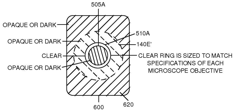
Fig. 10E--PHASE CONTRAST ILLUMINATION
