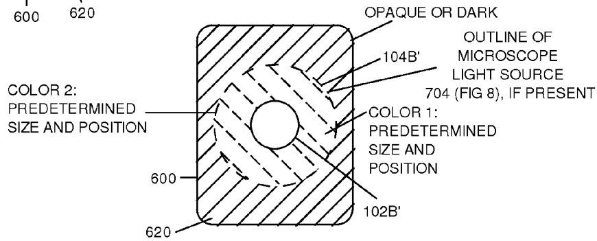
Fig. 10B--RHEINBERG ILLUMINATION
