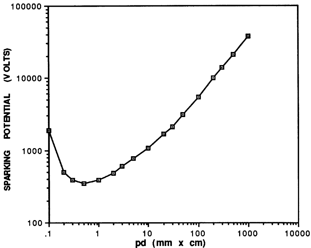
Fig. 5 Prior Art—Paschen's Law
